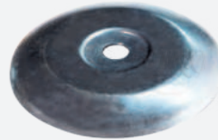
STEEL CAP FKK Ref. : 229.008 Outside Diameter : 104 Inside Diameter : 12,5 Height : 11/10
